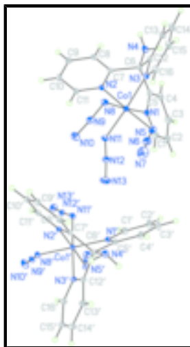
Fig. 1. Two molecules in the asymmetric unit of the title compound with displacement ellipsoids shown at 30 % probability for non-H atoms.
